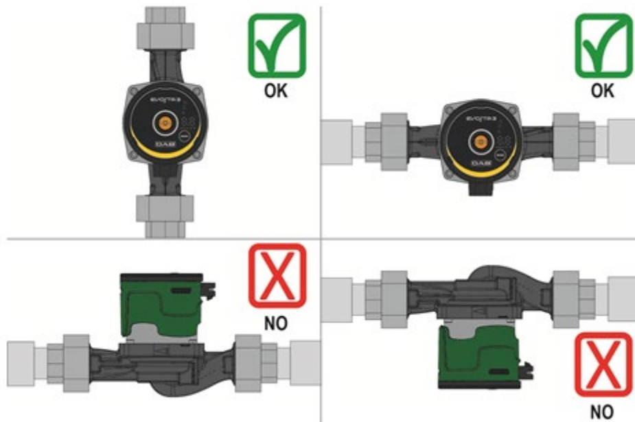
Figure 3: Assembly position
