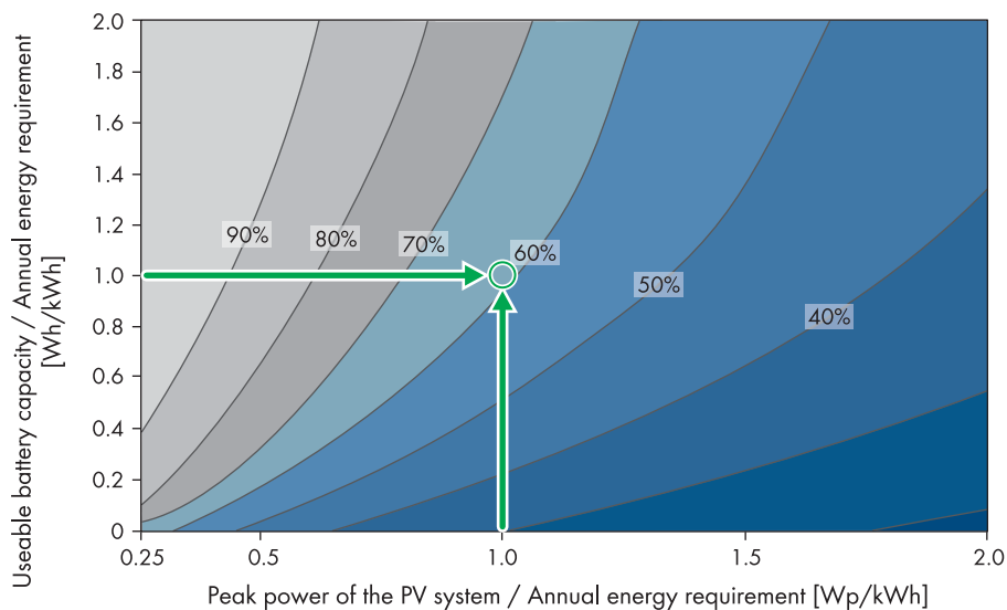
Figure 2: Estimation of self-consumption quota with intermediate storage
