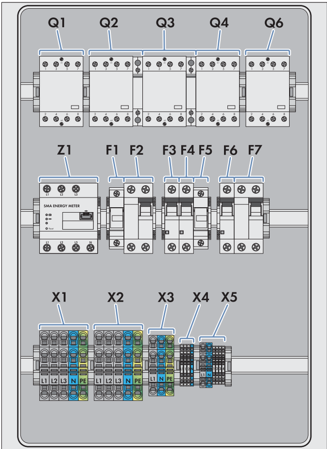
Figure 13: Configuration suggestion for single-phase automatic transfer switch with all-pole disconnection (e.g. for Germany)
