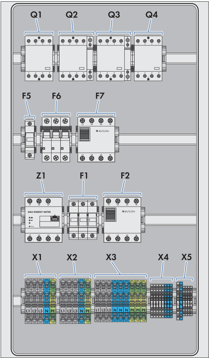
Figure 14: Configuration suggestion for three-phase automatic transfer switch with all-pole disconnection (e. g. for Germany)
