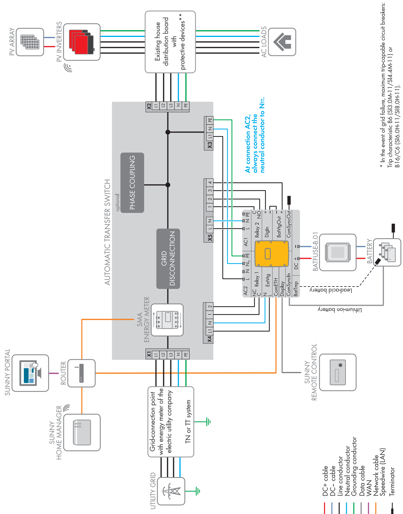
Figure 10: Circuitry overview of a single-phase battery-backup system without all-pole disconnection (e.g. for Australia)
