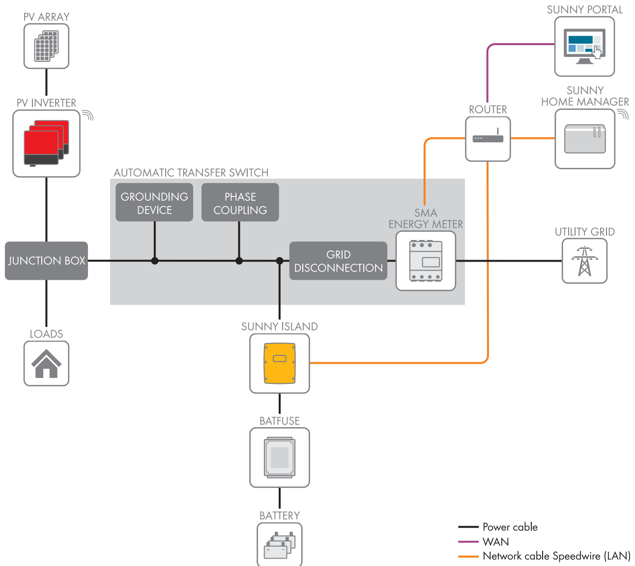
Figure 1: Overview of an SMA Flexible Storage System with battery-backup function
