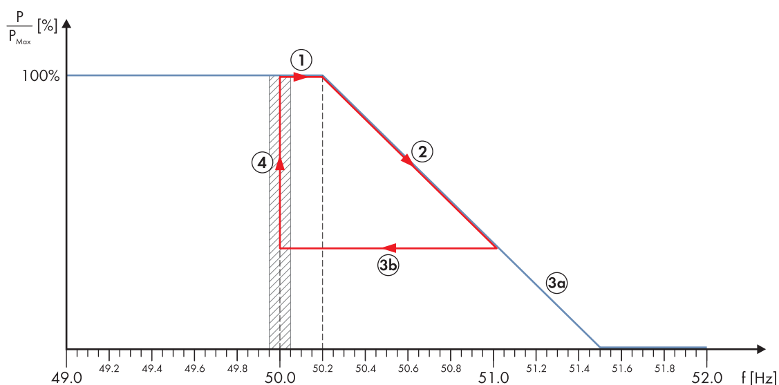
Figure 3: Suggestion for frequency-dependent active power limitation by the PV inverter (the frequencies are examples for Australia)
