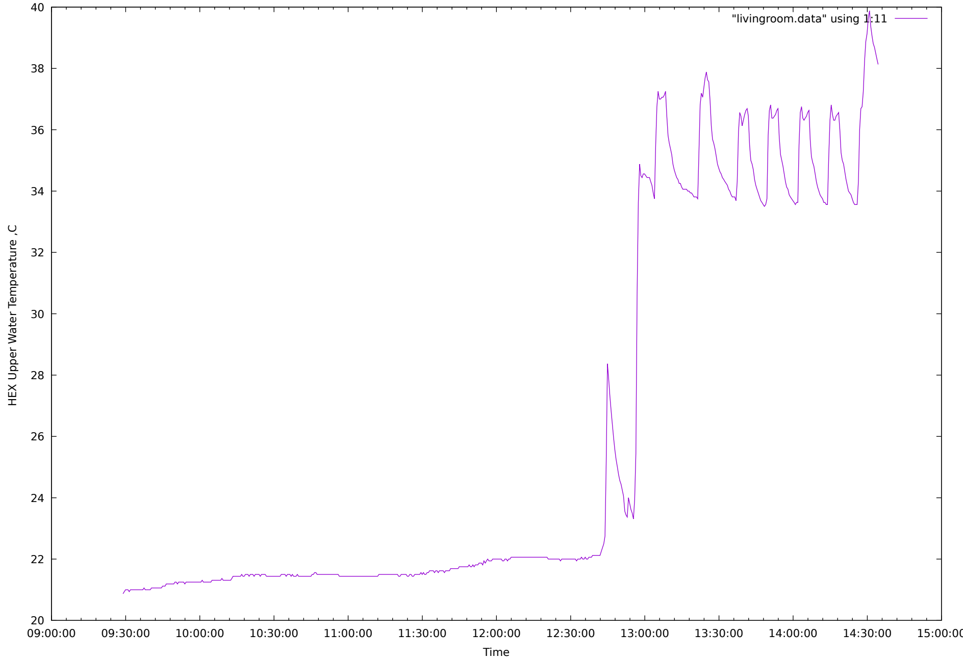
HEX Upper Water Temperature,C
