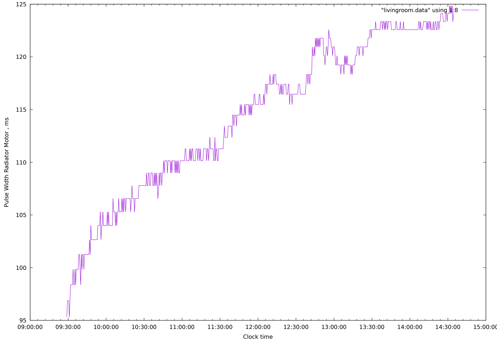
Pulse width Radiator Motor , ms
